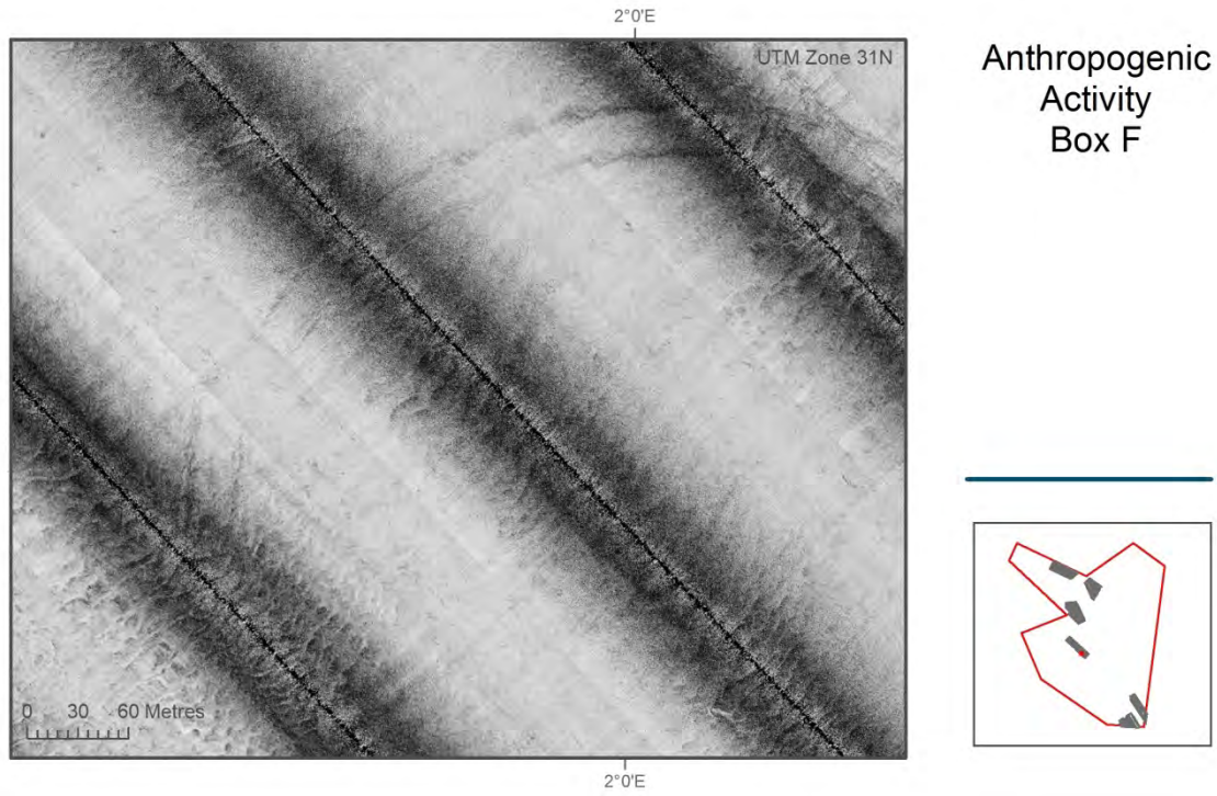
Figure 42. Side-scan sonar image at Box F showing trawl scarring of the seabed.
